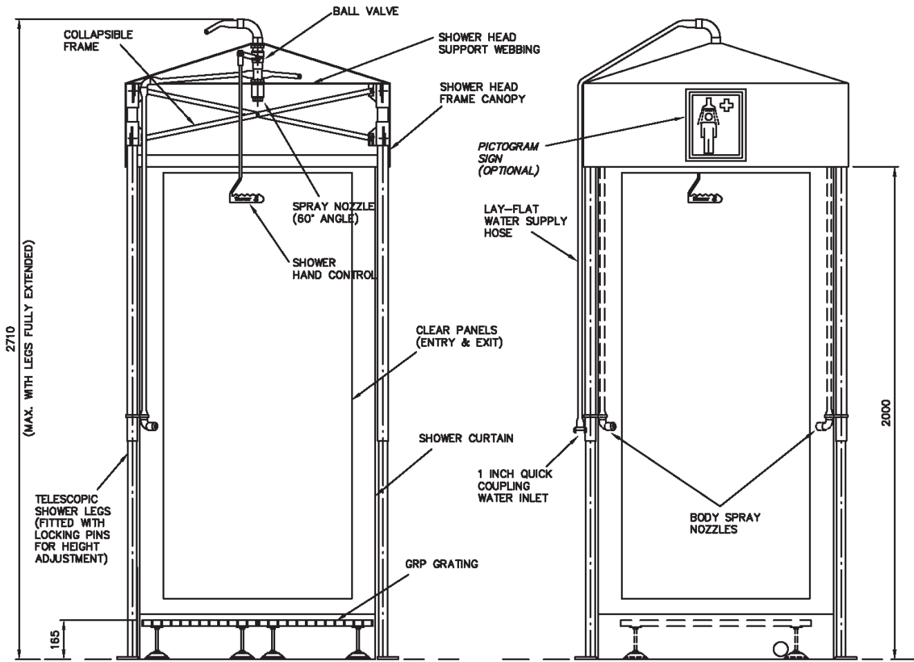
ELEVATION ON A-A
