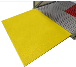
1215mm X 1000mm X 40mm for tank showers/cubicles with foot grating
