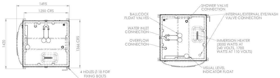
PLAN VIEWS WITH TANK LID OMITTED
