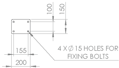
FIXING DETAIL VIEW
